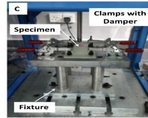
C. Impact Fixture
