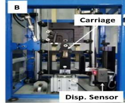
B. Carriage with Displacement Sensor
